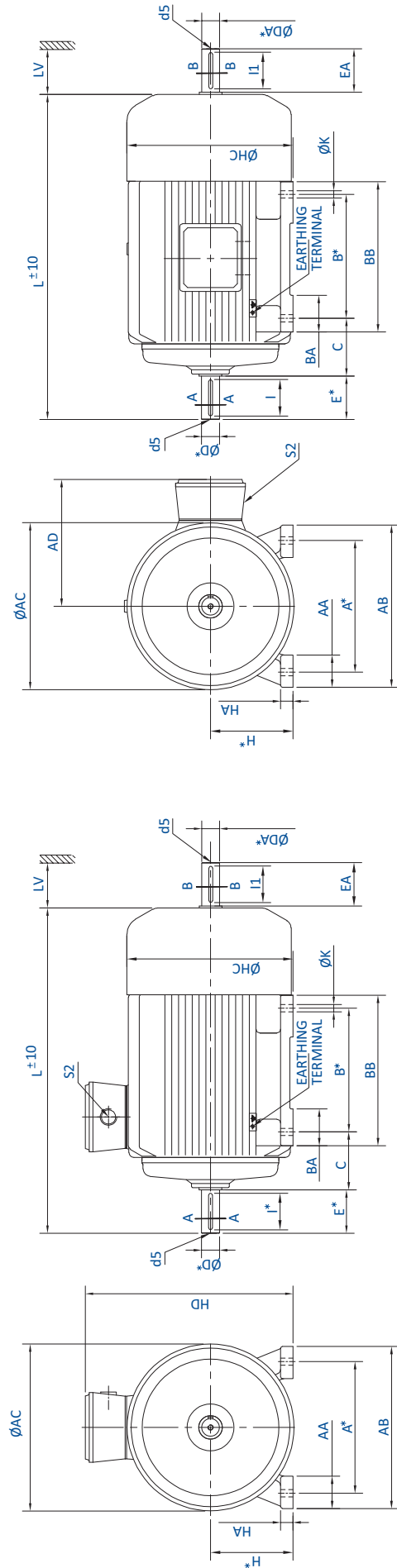
FRAME SIZE 71 TO 80
